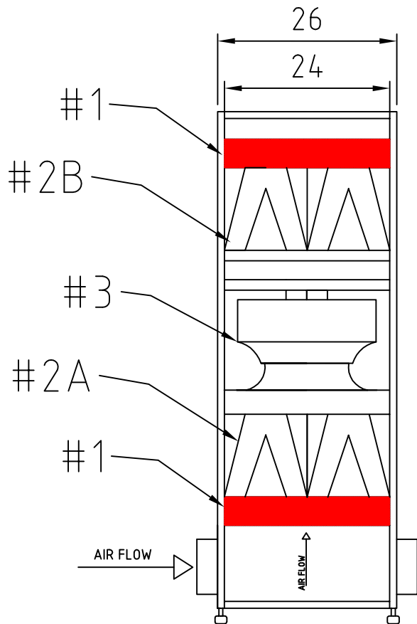
FRONT VIEW WITH OUT DOORS
